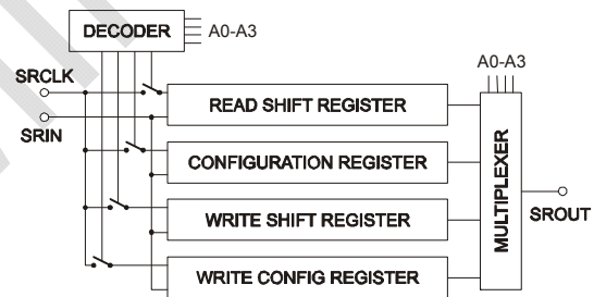
Figure 6. Sharing of Shift Register Signals
